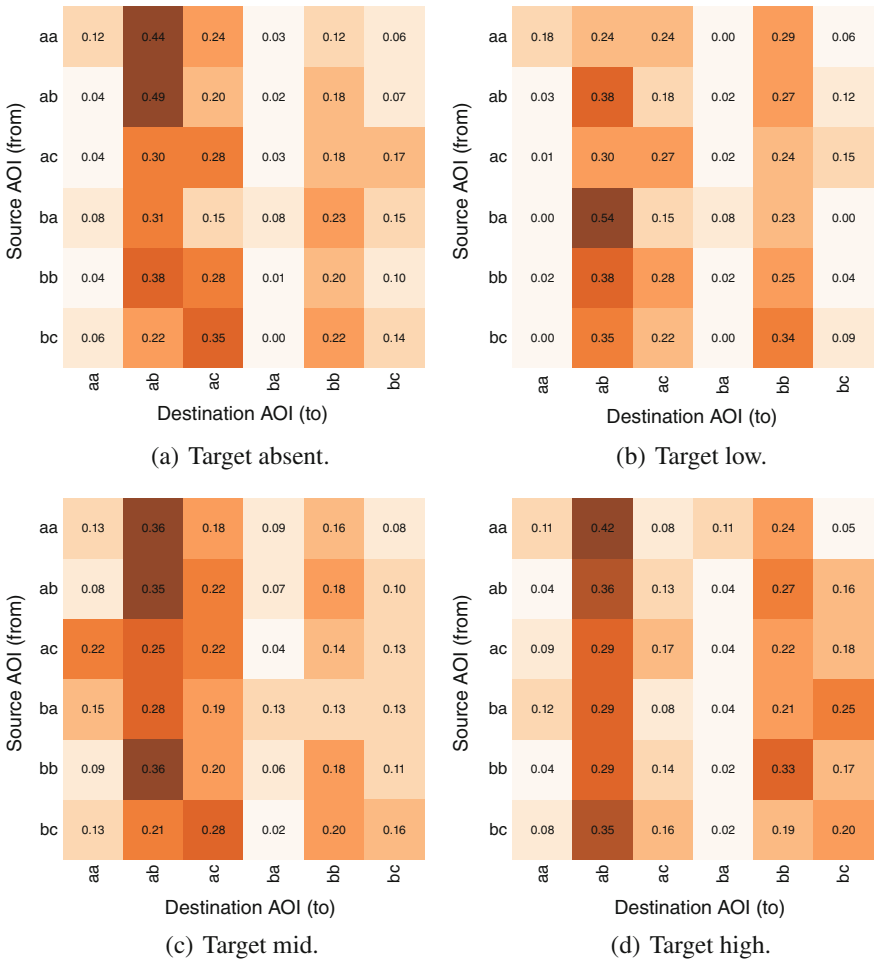
Fig. 15.8 Transition matrices
