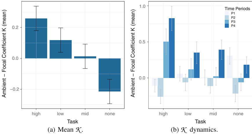
Fig. 15.6 Analysis of mean \mathcal{K} , \mathcal{K} dynamics, and transition entropy ( 2 \times 3 AOI grid)
