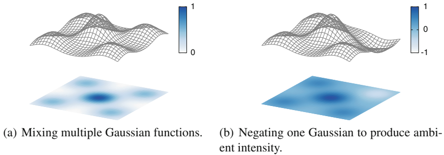
Fig. 14.8 Mixing Gaussian point spread functions to produce an ambient/focal heatmap. Two hypothetical fixations overlap in the center, with an additional fixation at each corner. Ambient intensity is modeled by negating the Gaussian function (at upper-right ), producing a valley instead of a peak
