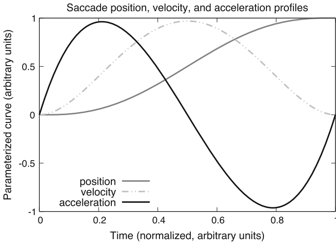
Fig. 12.2 Nonlinear blending function H(t) for position of calibration dot, modeled after a parametric saccade position model derived in turn from an idealized model of saccadic force-time function assumed by Abrams et al.'s (1989) symmetric-impulse variability function: scaled position 60H(t) , velocity 31\dot{H}(t) , and acceleration 10\ddot{H}(t)
