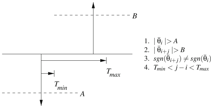
Fig. 13.8 Acceleration thresholding
